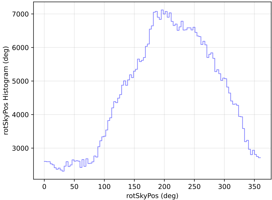
too_elab_heavy_r64_d2_ugrizy_v3.4_10yrs All sky i band: rotSkyPos Histogram
