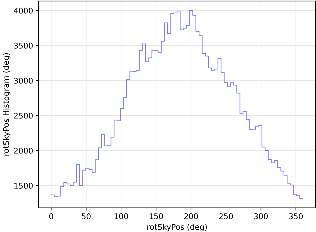
too_elab_heavy_r64_d2_ugrizy_v3.4_10yrs All sky g band: rotSkyPos Histogram
