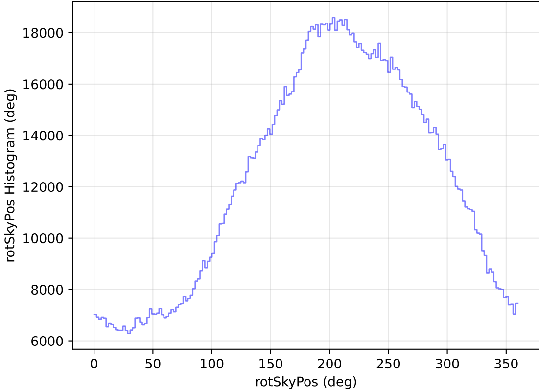
too_elab_heavy_r64_d2_ugrizy_v3.4_10yrs All sky all bands: rotSkyPos Histogram
