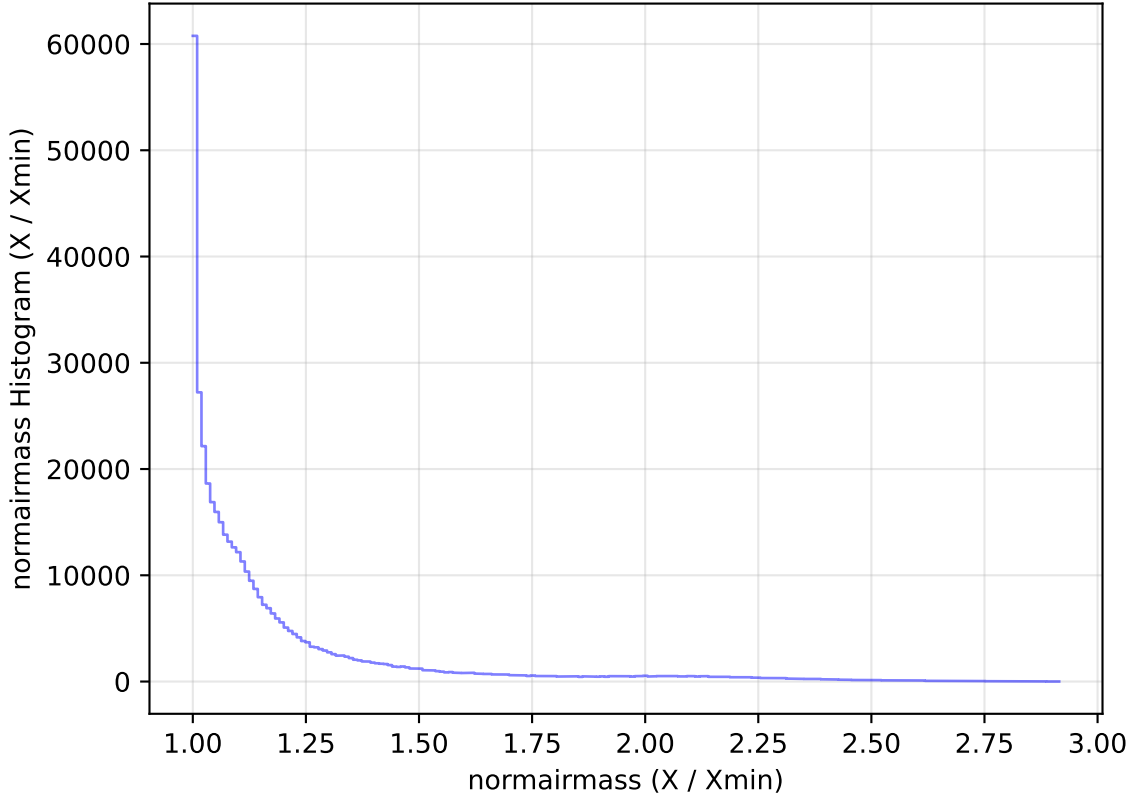
too_elab_heavy_r64_d2_ugrizy_v3.4_10yrs WFD z band: normairmass Histogram
