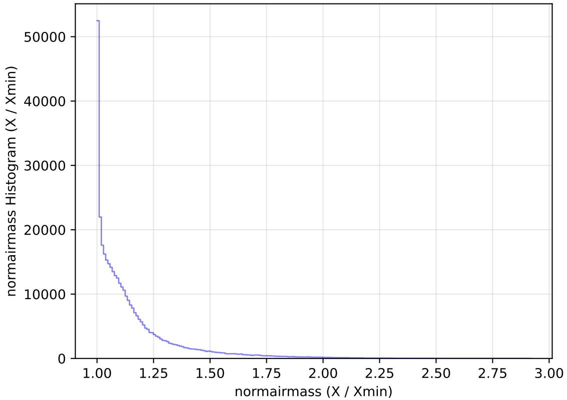
too_elab_heavy_r64_d2_ugrizy_v3.4_10yrs WFD y band: normairmass Histogram
