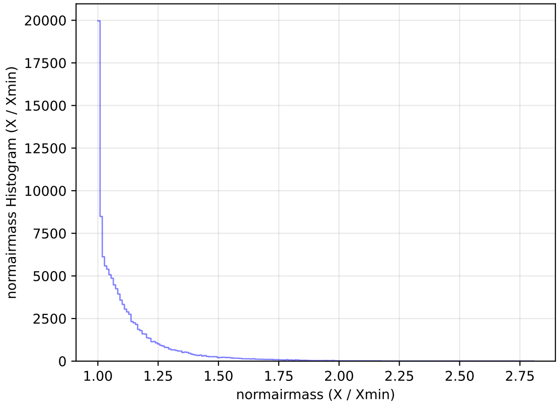
too_elab_heavy_r64_d2_ugrizy_v3.4_10yrs WFD u band: normairmass Histogram
