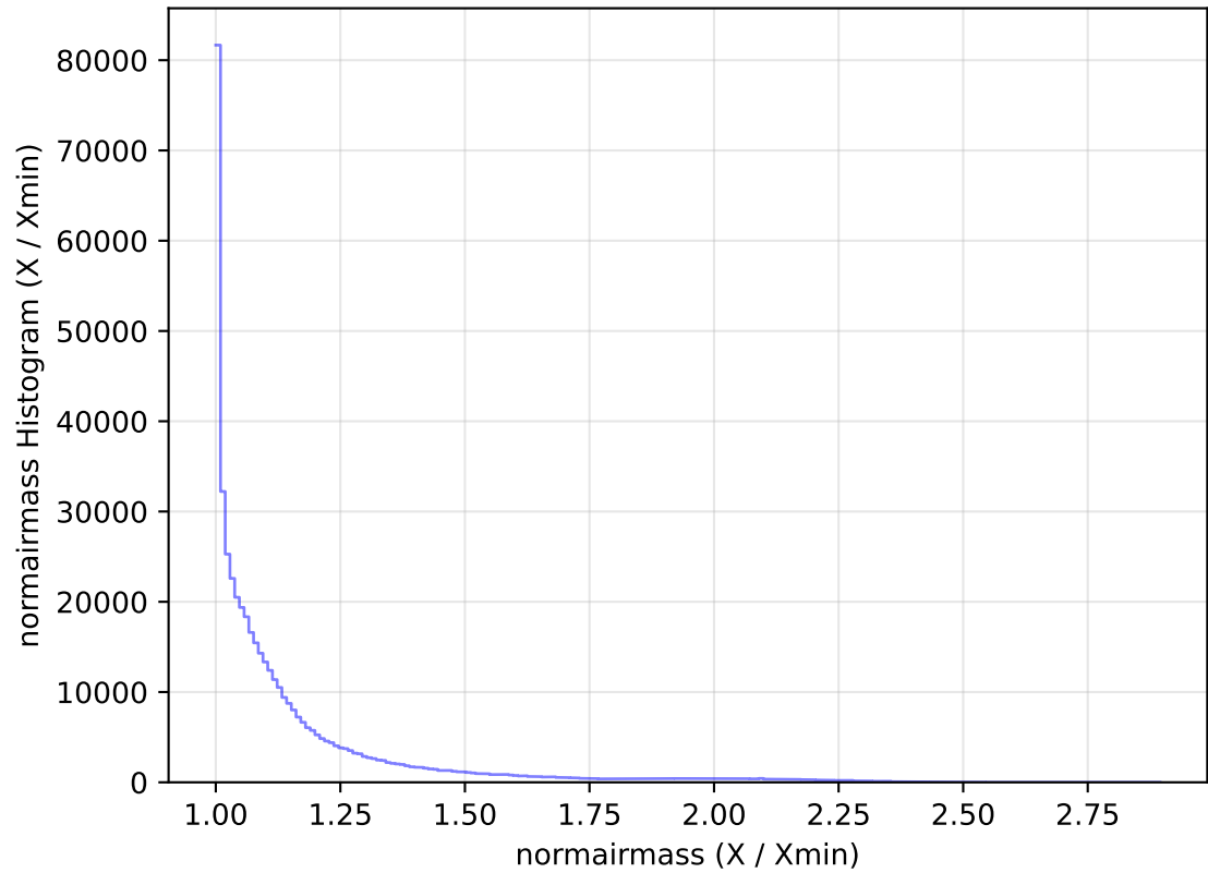
too_elab_heavy_r64_d2_ugrizy_v3.4_10yrs WFD r band: normairmass Histogram
