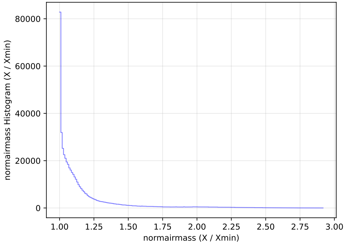
too_elab_heavy_r64_d2_ugrizy_v3.4_10yrs WFD i band: normairmass Histogram
