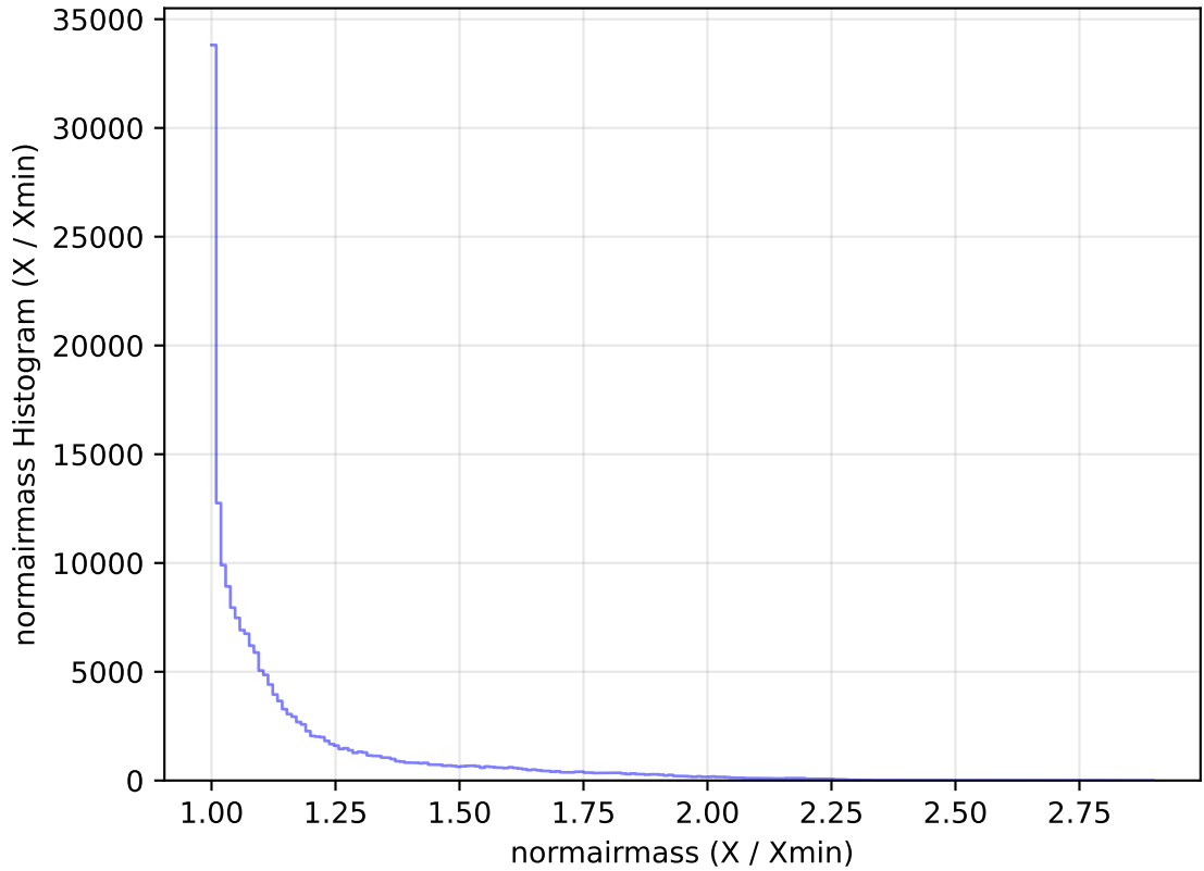
too_elab_heavy_r64_d2_ugrizy_v3.4_10yrs WFD g band: normairmass Histogram
