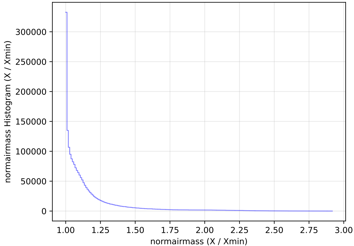
too_elab_heavy_r64_d2_ugrizy_v3.4_10yrs WFD all bands: normairmass Histogram
