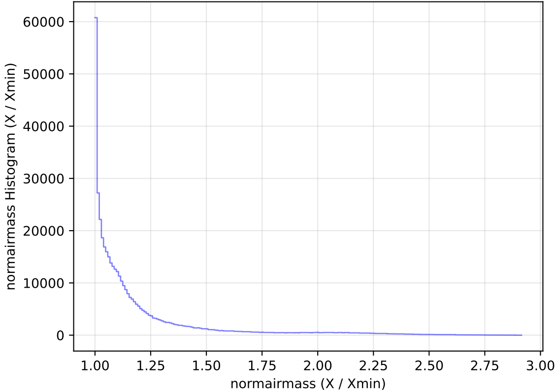
too_elab_heavy_r64_d2_ugrizy_v3.4_10yrs All sky z band: normairmass Histogram
