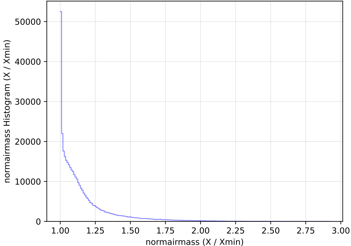
too_elab_heavy_r64_d2_ugrizy_v3.4_10yrs All sky y band: normairmass Histogram
