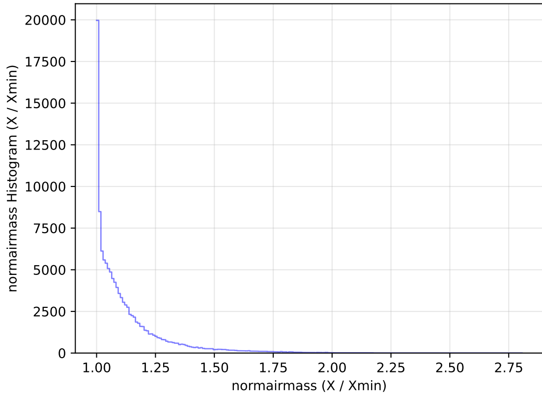
too_elab_heavy_r64_d2_ugrizy_v3.4_10yrs All sky u band: normairmass Histogram
