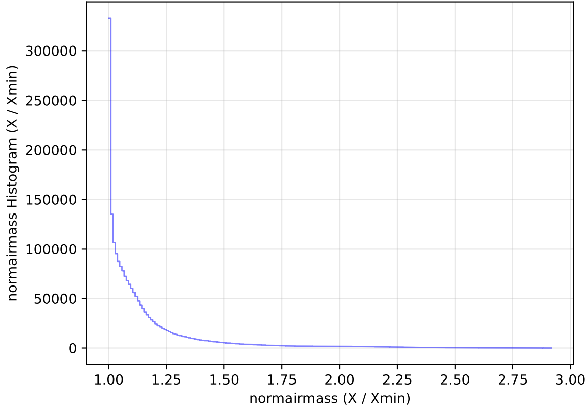
too_elab_heavy_r64_d2_ugrizy_v3.4_10yrs All sky all bands: normairmass Histogram
