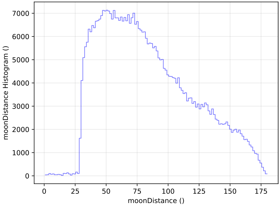
too_elab_heavy_r64_d2_ugrizy_v3.4_10yrs WFD z band: moonDistance Histogram
