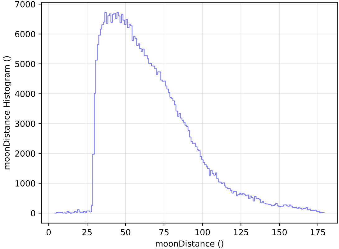
too_elab_heavy_r64_d2_ugrizy_v3.4_10yrs WFD y band: moonDistance Histogram
