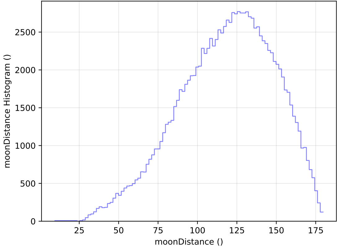
too_elab_heavy_r64_d2_ugrizy_v3.4_10yrs WFD u band: moonDistance Histogram
