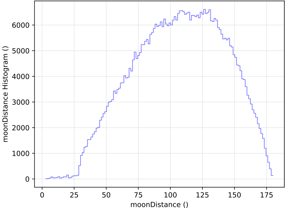
too_elab_heavy_r64_d2_ugrizy_v3.4_10yrs WFD r band: moonDistance Histogram
