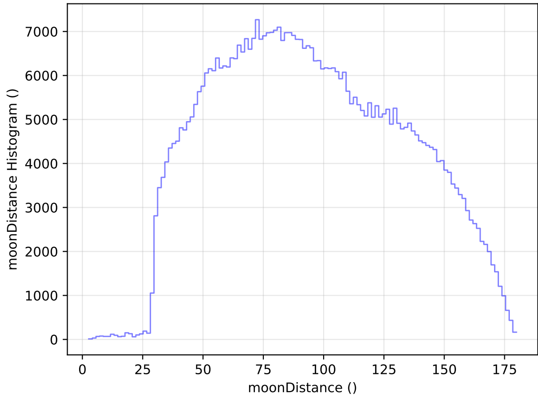
too_elab_heavy_r64_d2_ugrizy_v3.4_10yrs WFD i band: moonDistance Histogram
