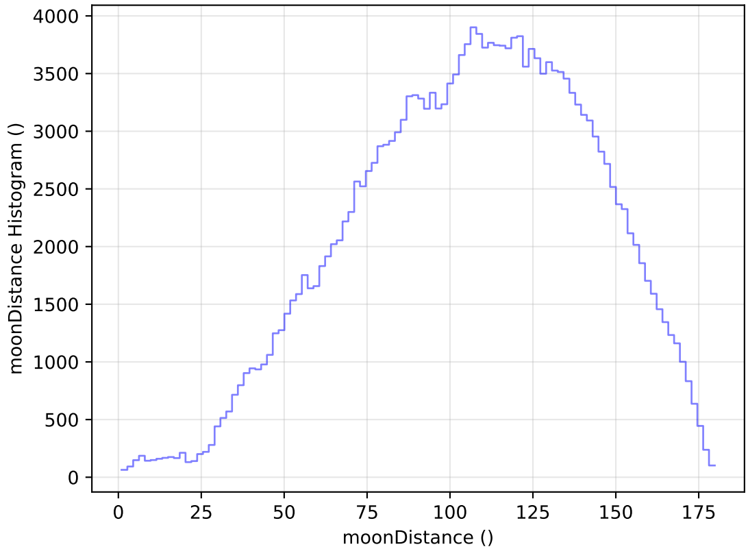
too_elab_heavy_r64_d2_ugrizy_v3.4_10yrs WFD g band: moonDistance Histogram
