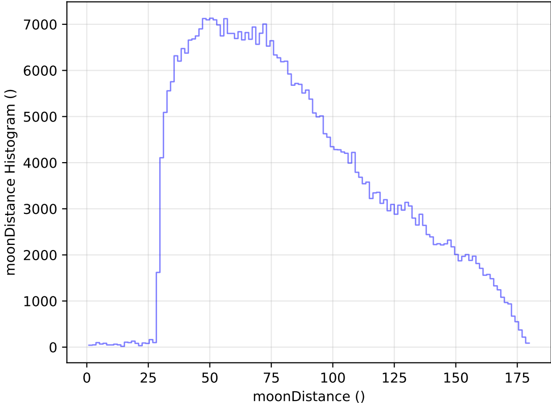
too_elab_heavy_r64_d2_ugrizy_v3.4_10yrs All sky z band: moonDistance Histogram
