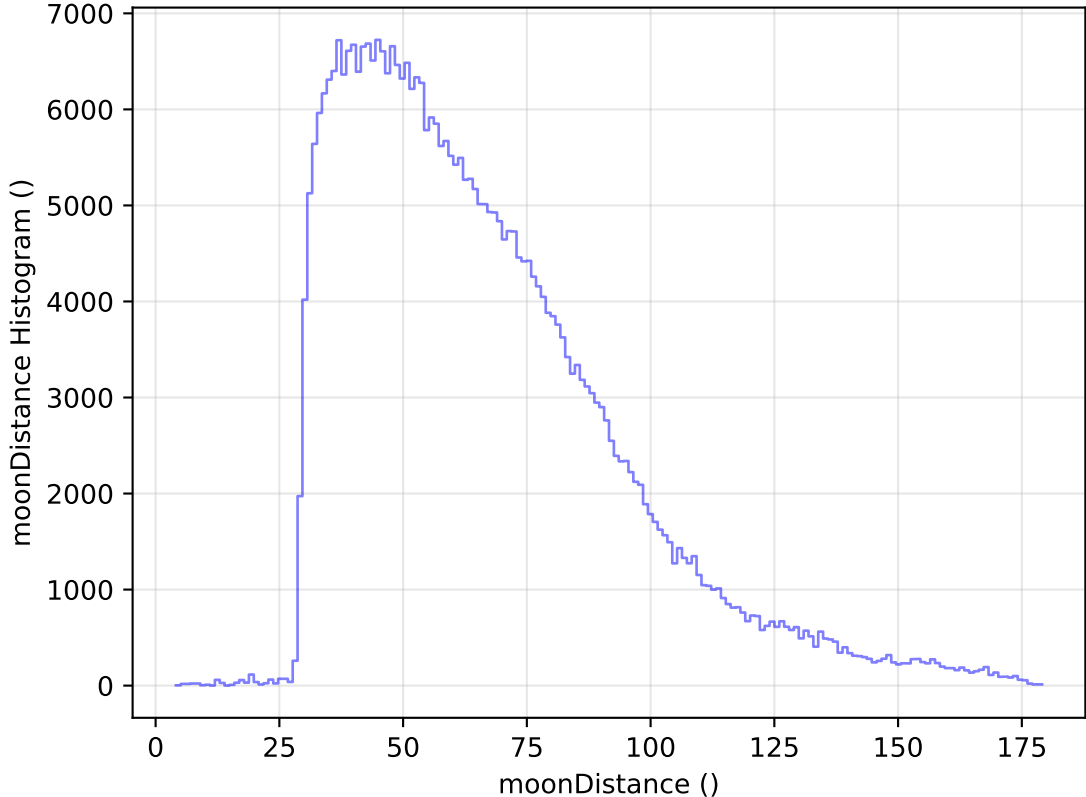
too_elab_heavy_r64_d2_ugrizy_v3.4_10yrs All sky y band: moonDistance Histogram
