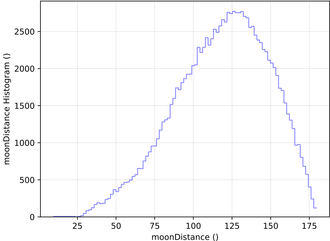
too_elab_heavy_r64_d2_ugrizy_v3.4_10yrs All sky u band: moonDistance Histogram
