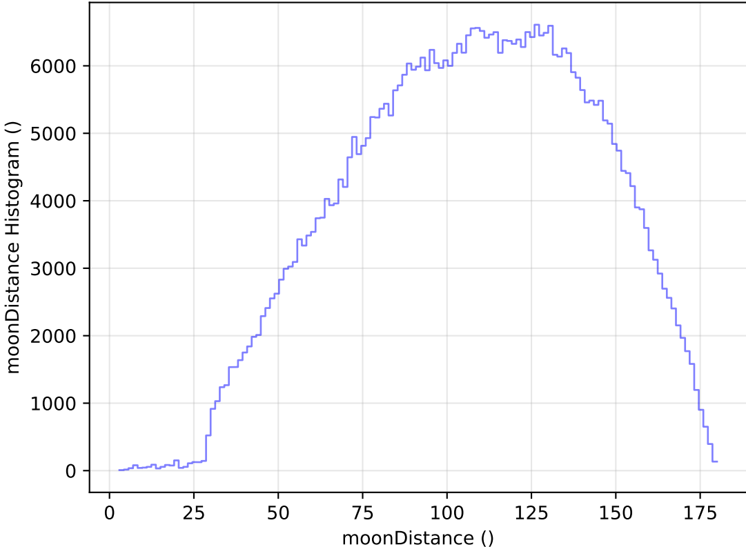
too_elab_heavy_r64_d2_ugrizy_v3.4_10yrs All sky r band: moonDistance Histogram
