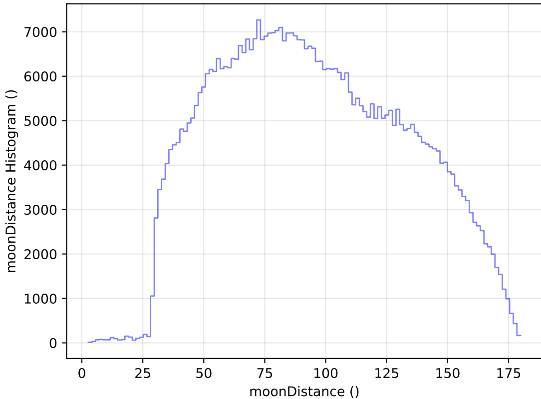
too_elab_heavy_r64_d2_ugrizy_v3.4_10yrs All sky i band: moonDistance Histogram
