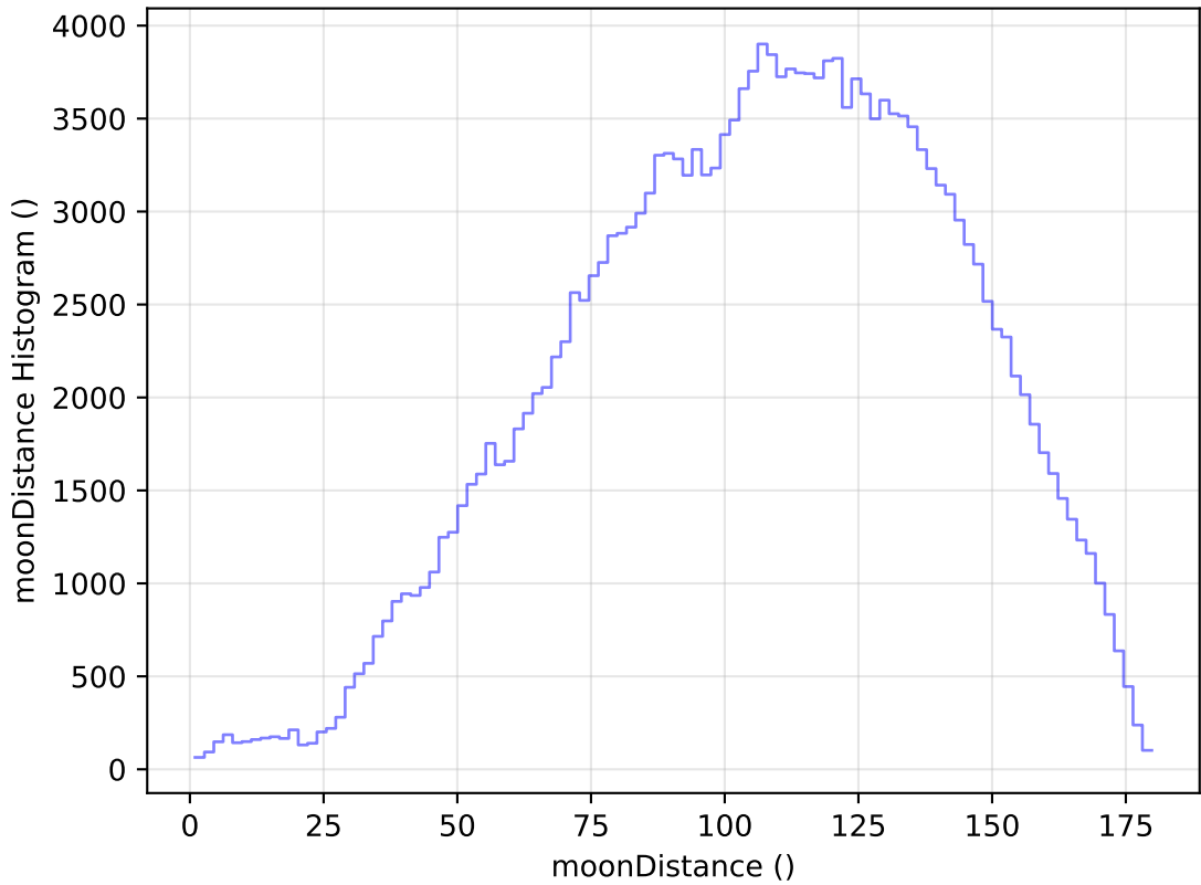
too_elab_heavy_r64_d2_ugrizy_v3.4_10yrs All sky g band: moonDistance Histogram
