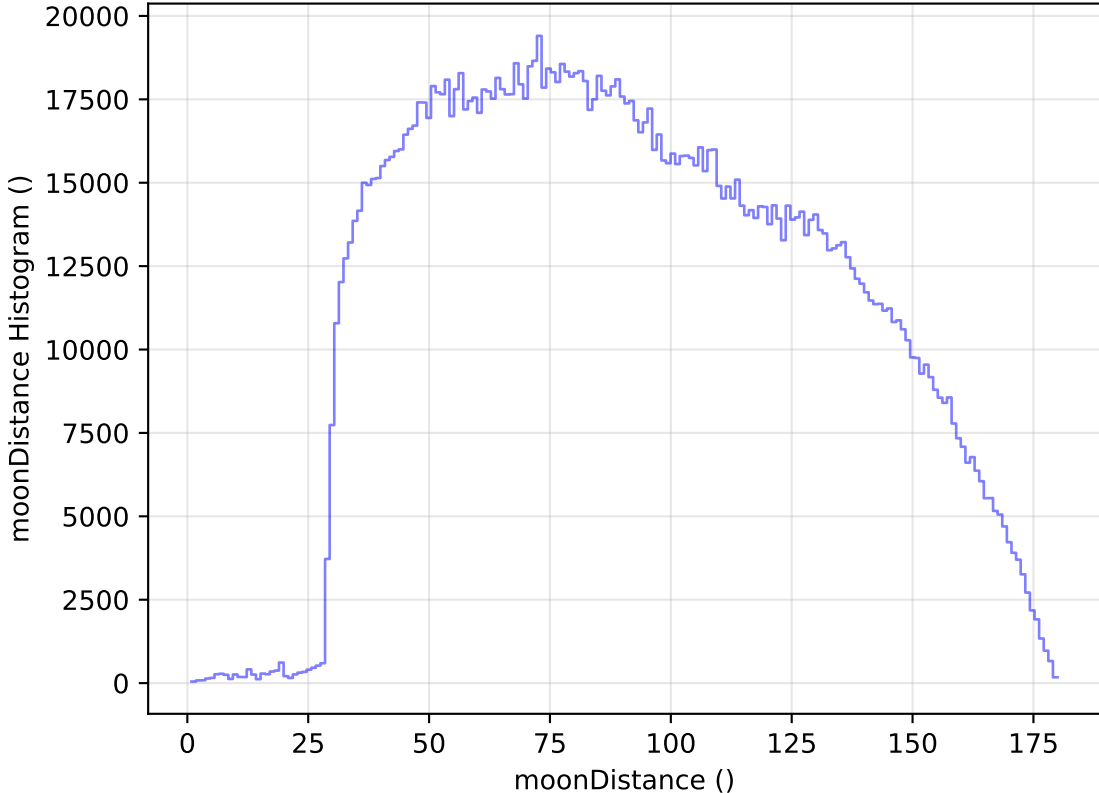
too_elab_heavy_r64_d2_ugrzy_v3.4_10yrs All sky all bands: moonDistance Histogram
