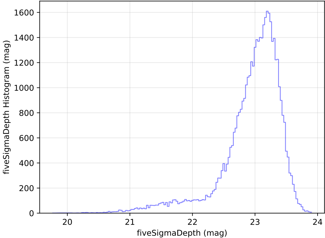
too_elab_heavy_r64_d2_ugrizy_v3.4_10yrs Yr 1 z band: fiveSigmaDepth Histogram
