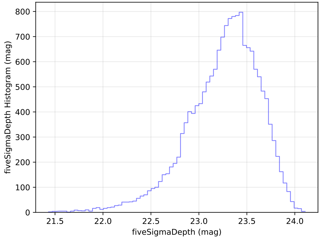
too_elab_heavy_r64_d2_ugrizy_v3.4_10yrs Yr 1 u band: fiveSigmaDepth Histogram
