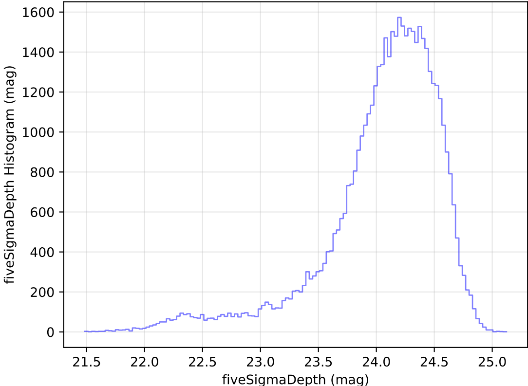
too_elab_heavy_r64_d2_ugrizy_v3.4_10yrs Yr 1 r band: fiveSigmaDepth Histogram
