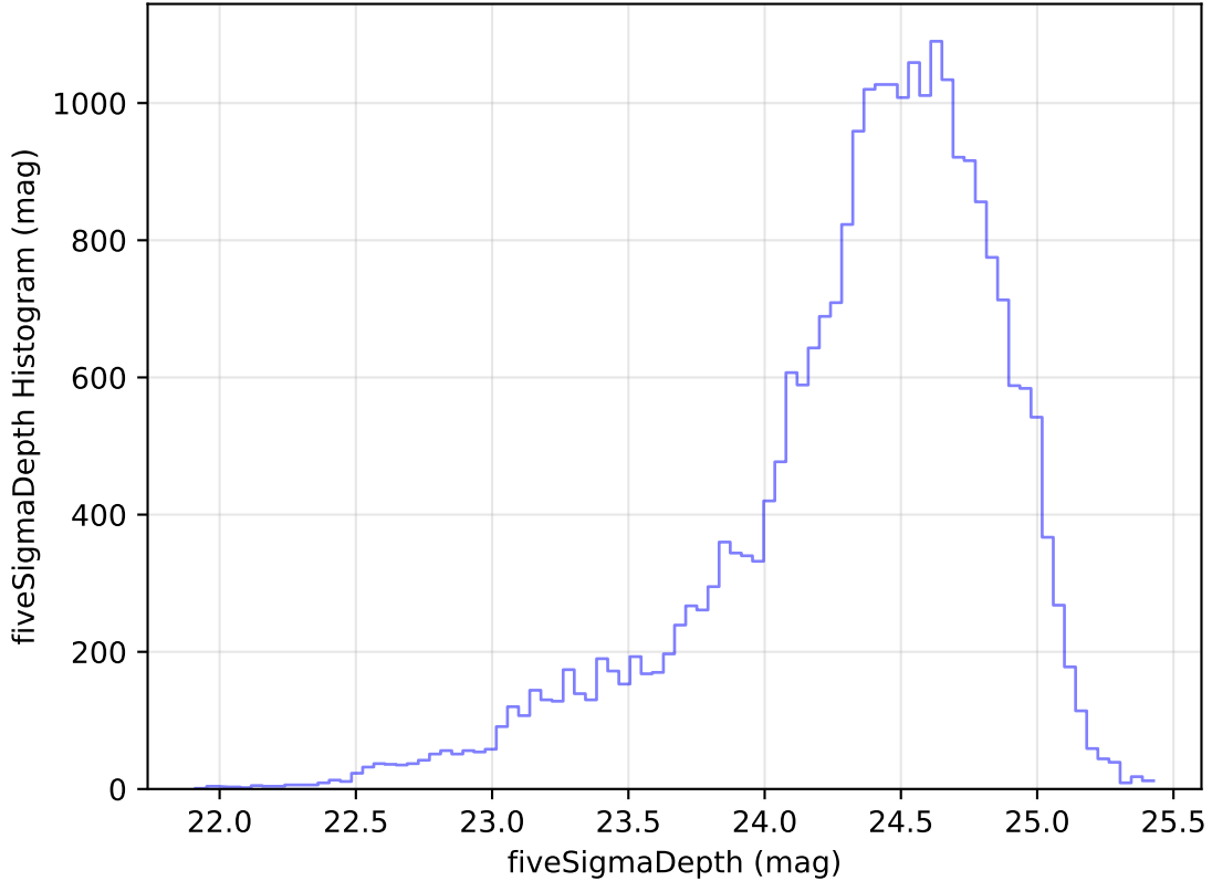
too_elab_heavy_r64_d2_ugrizy_v3.4_10yrs Yr 1 g band: fiveSigmaDepth Histogram
