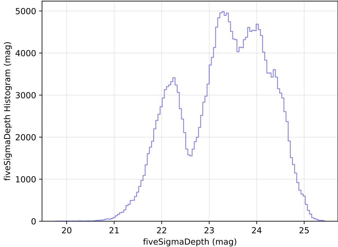
too_elab_heavy_r64_d2_ugrizy_v3.4_10yrs Yr 1 all bands: fiveSigmaDepth Histogram
