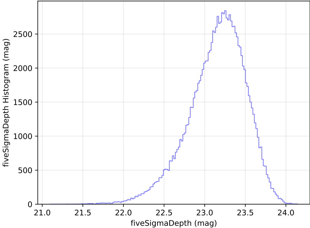
too_elab_heavy_r64_d2_ugrizy_v3.4_10yrs WFD u band: fiveSigmaDepth Histogram
