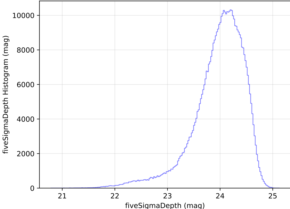
too_elab_heavy_r64_d2_ugrizy_v3.4_10yrs WFD r band: fiveSigmaDepth Histogram
