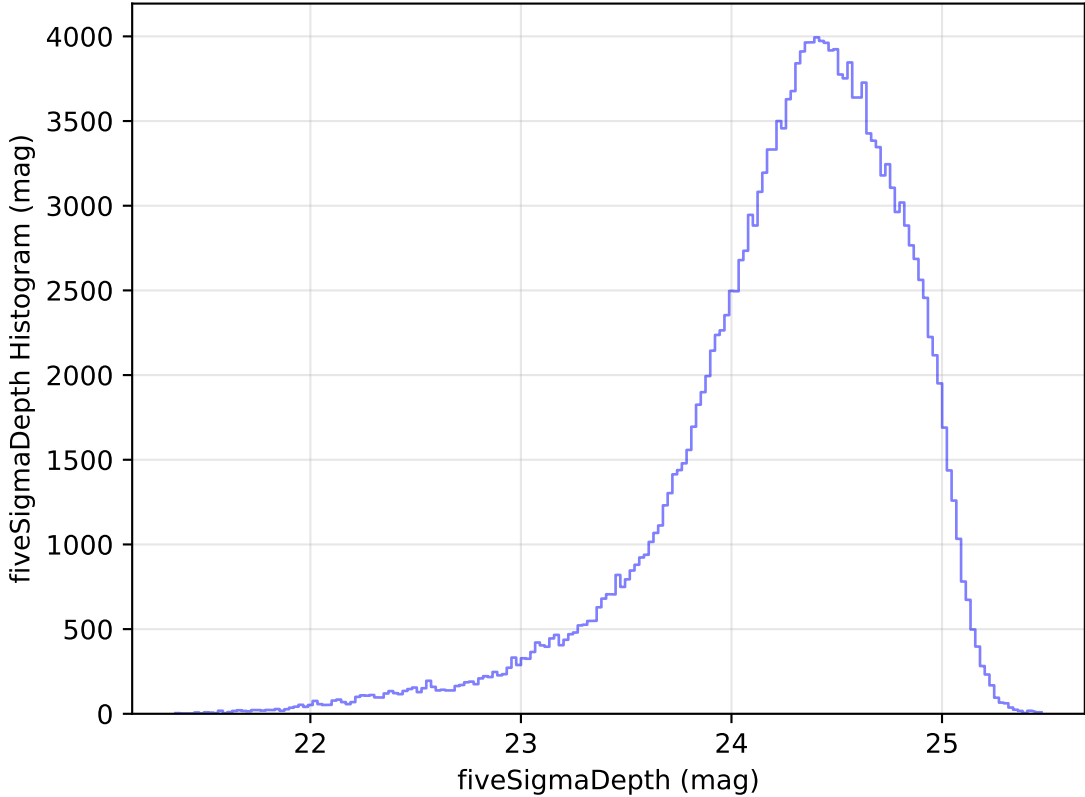
too_elab_heavy_r64_d2_ugrizy_v3.4_10yrs WFD g band: fiveSigmaDepth Histogram
