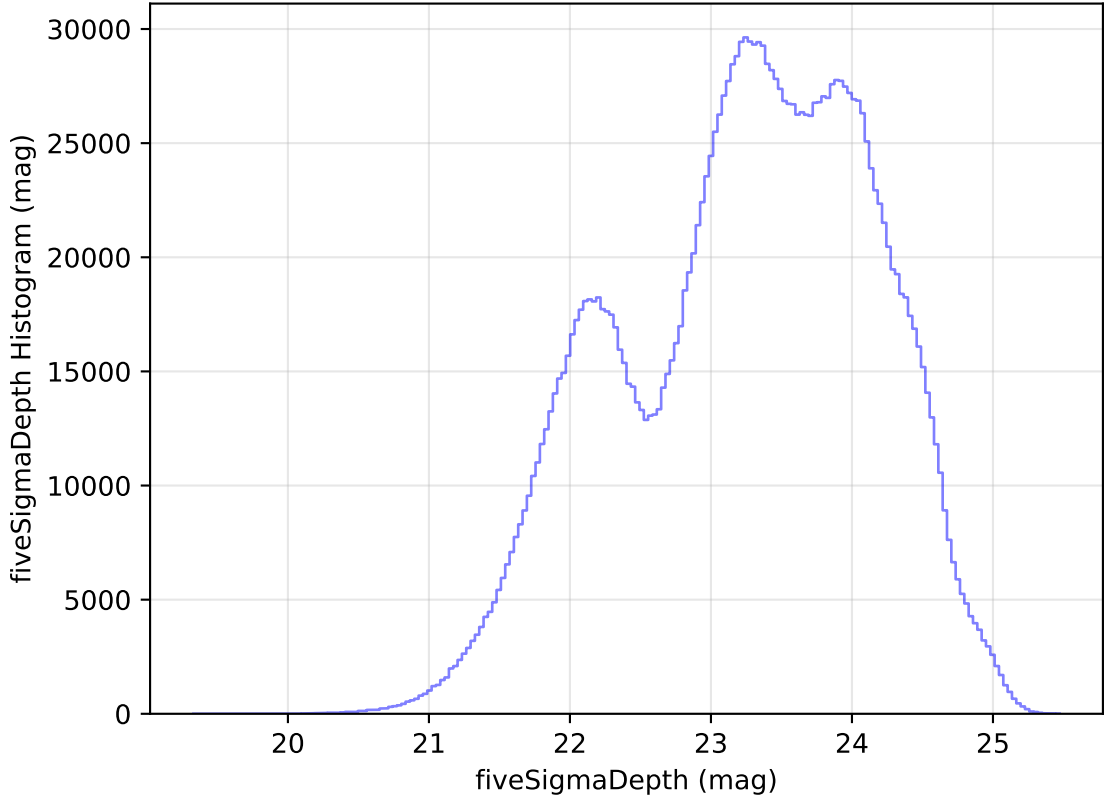
too_elab_heavy_r64_d2_ugrizy_v3.4_10yrs WFD all bands: fiveSigmaDepth Histogram
