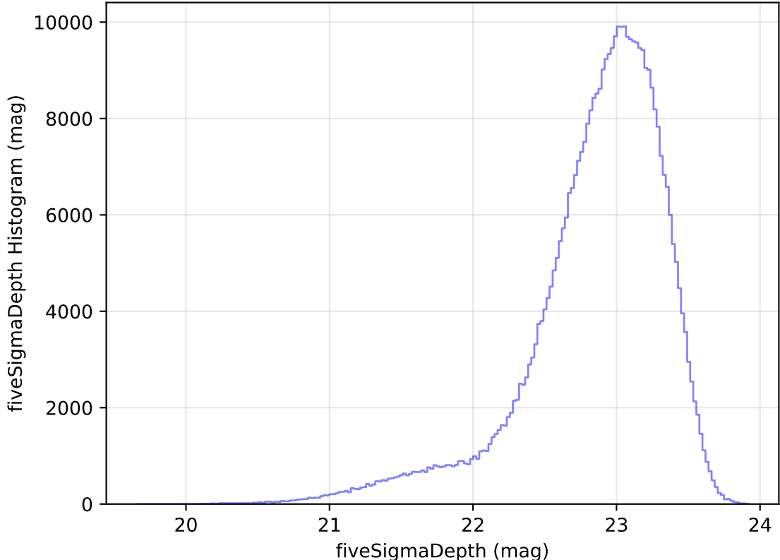
too_elab_heavy_r64_d2_ugrizy_v3.4_10yrs All sky z band: fiveSigmaDepth Histogram
