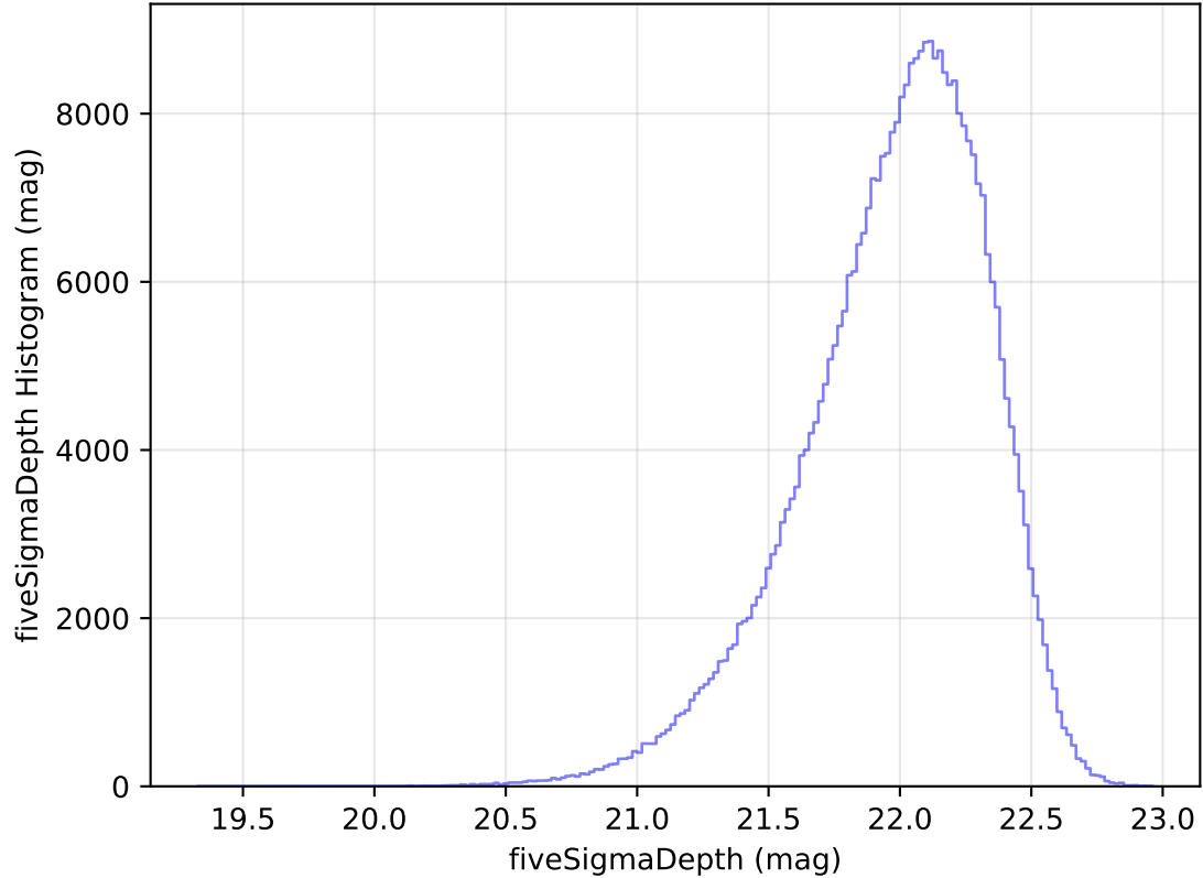
too_elab_heavy_r64_d2_ugrizy_v3.4_10yrs All sky y band: fiveSigmaDepth Histogram
