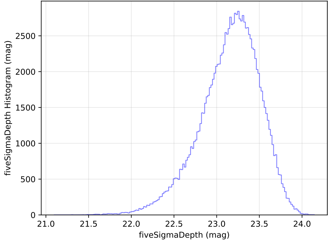
too_elab_heavy_r64_d2_ugrizy_v3.4_10yrs All sky u band: fiveSigmaDepth Histogram
