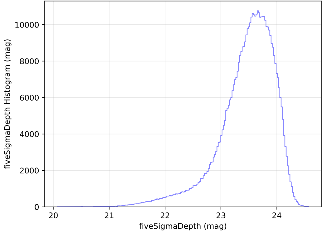
too_elab_heavy_r64_d2_ugrizy_v3.4_10yrs All sky i band: fiveSigmaDepth Histogram
