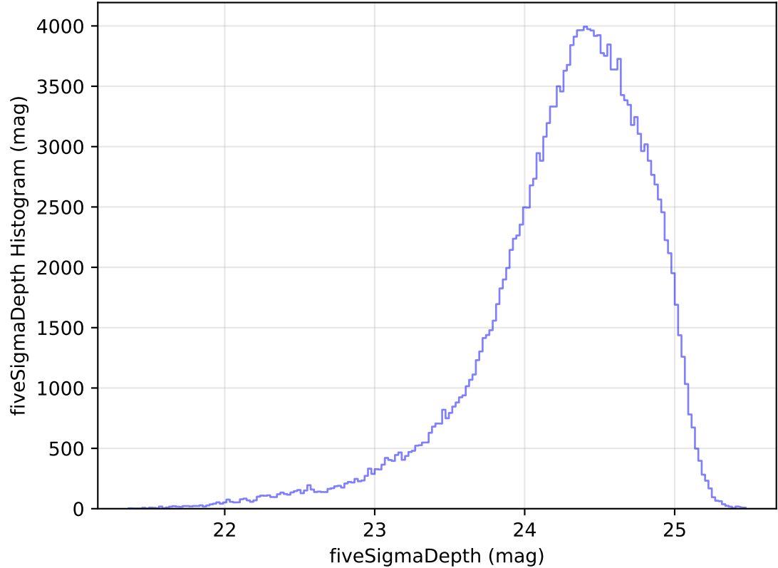
too_elab_heavy_r64_d2_ugrizy_v3.4_10yrs All sky g band: fiveSigmaDepth Histogram
