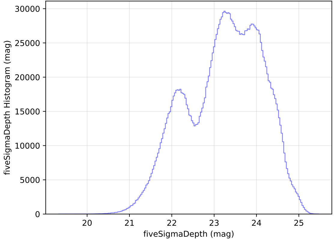
too_elab_heavy_r64_d2_ugrizy_v3.4_10yrs All sky all bands: fiveSigmaDepth Histogram
