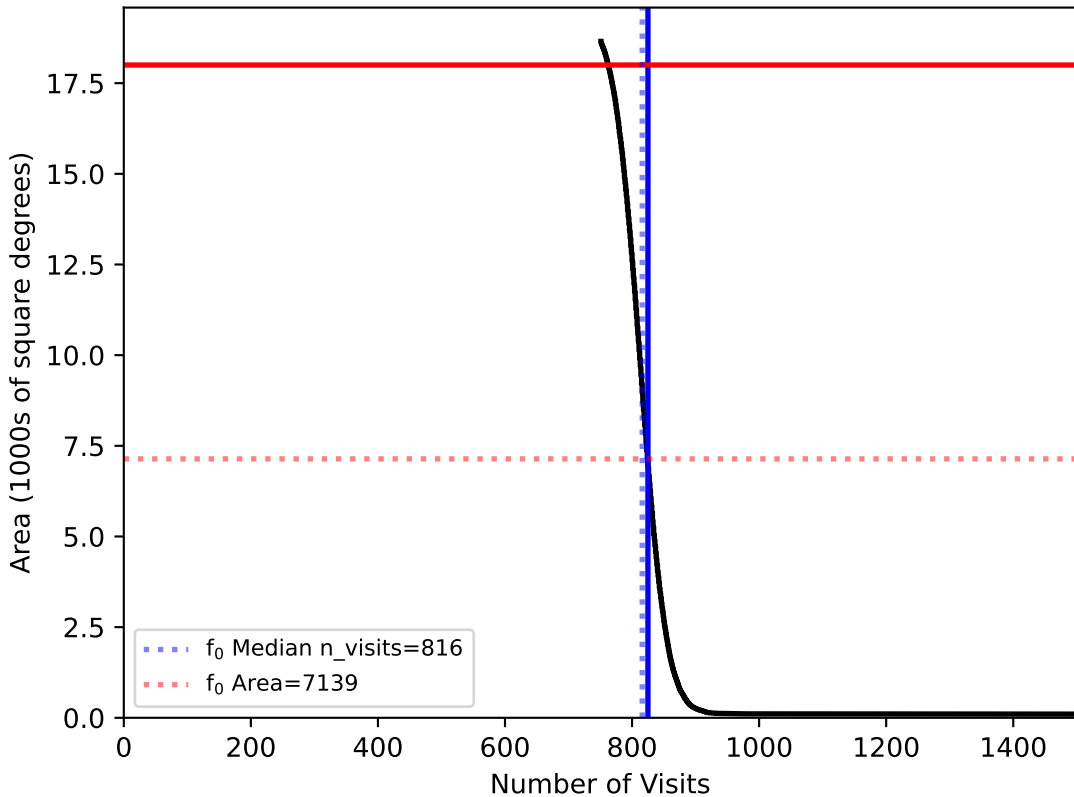
too_elab_heavy_r64_d2_ugrizy_v3.4_10yrs WFD: f0
