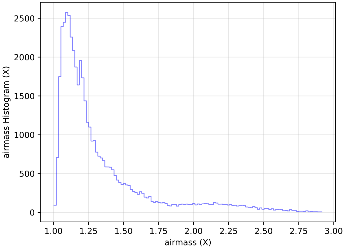
too_elab_heavy_r64_d2_ugrizy_v3.4_10yrs Yr 1 z band: airmass Histogram
