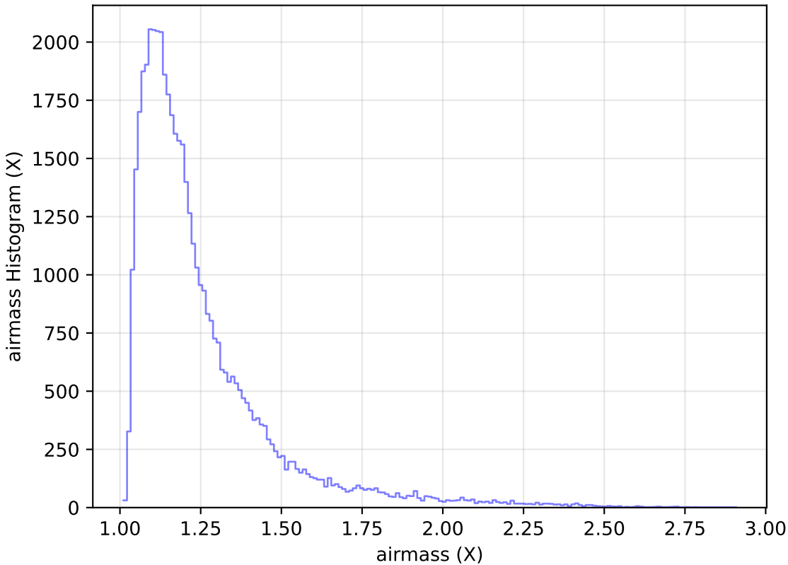
too_elab_heavy_r64_d2_ugrizy_v3.4_10yrs Yr 1 y band: airmass Histogram
