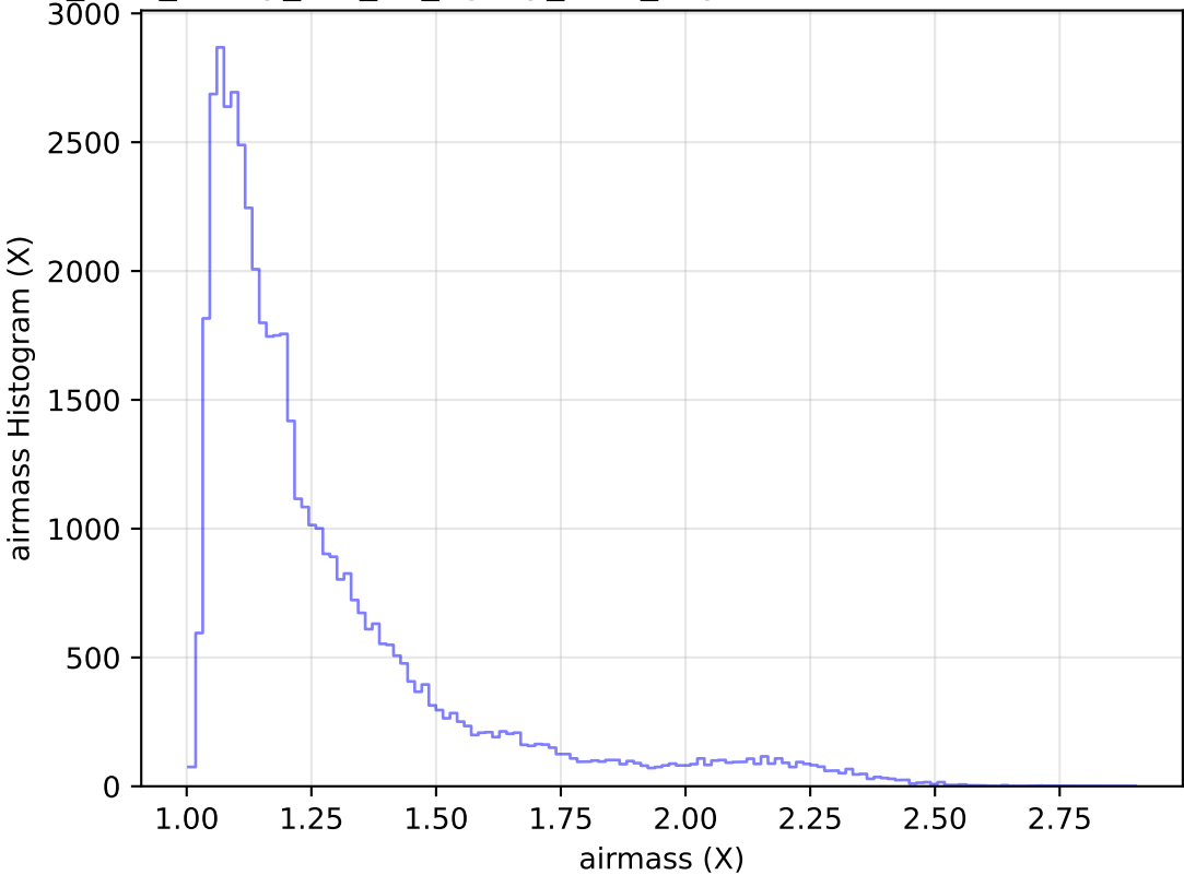
too_elab_heavy_r64_d2_ugrizy_v3.4_10yrs Yr 1 r band: airmass Histogram
