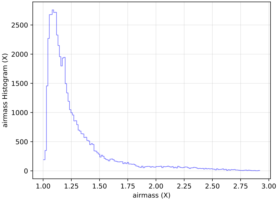
too_elab_heavy_r64_d2_ugrizy_v3.4_10yrs Yr 1 i band: airmass Histogram
