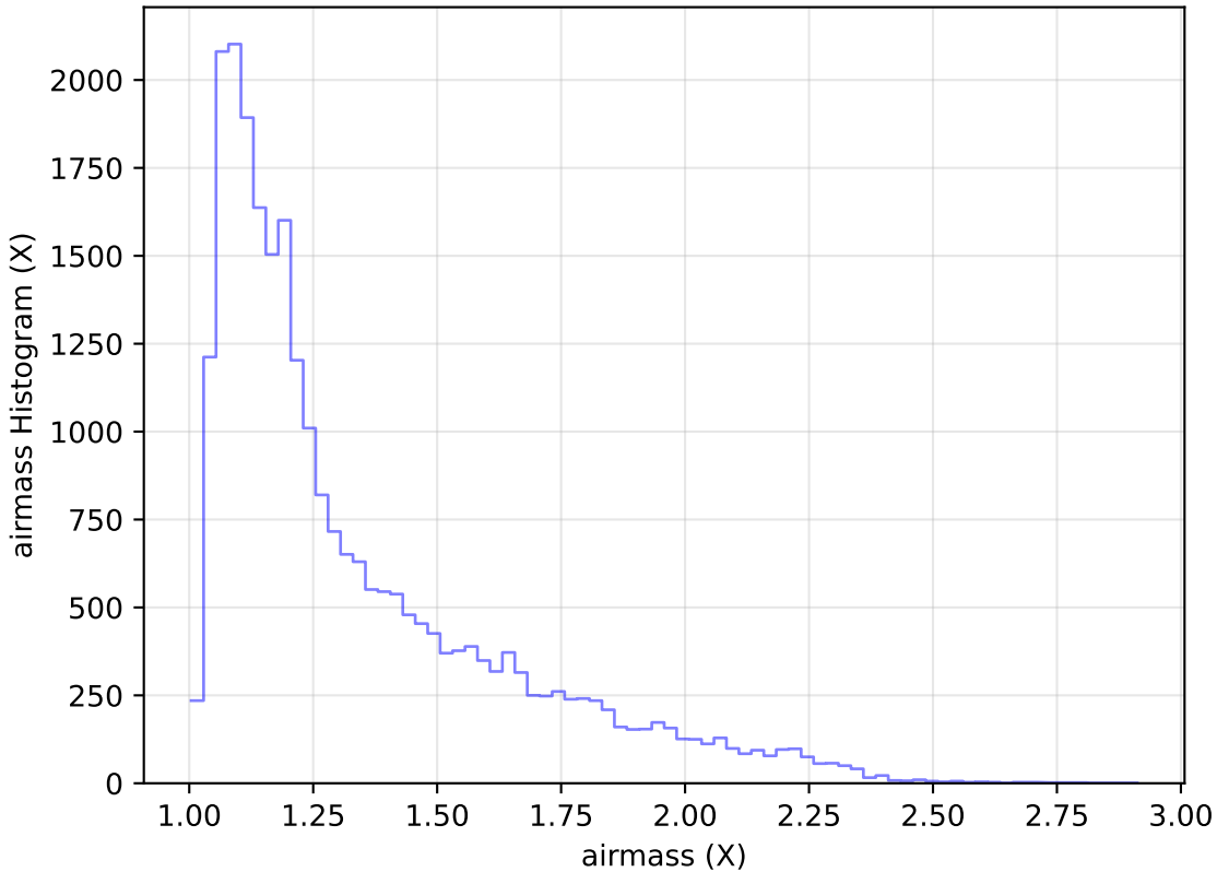
too_elab_heavy_r64_d2_ugrizy_v3.4_10yrs Yr 1 g band: airmass Histogram
