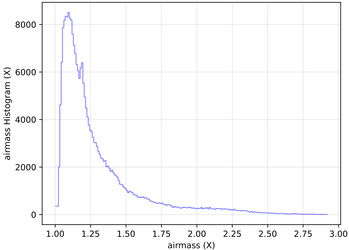
too_elab_heavy_r64_d2_ugrizy_v3.4_10yrs Yr 1 all bands: airmass Histogram
