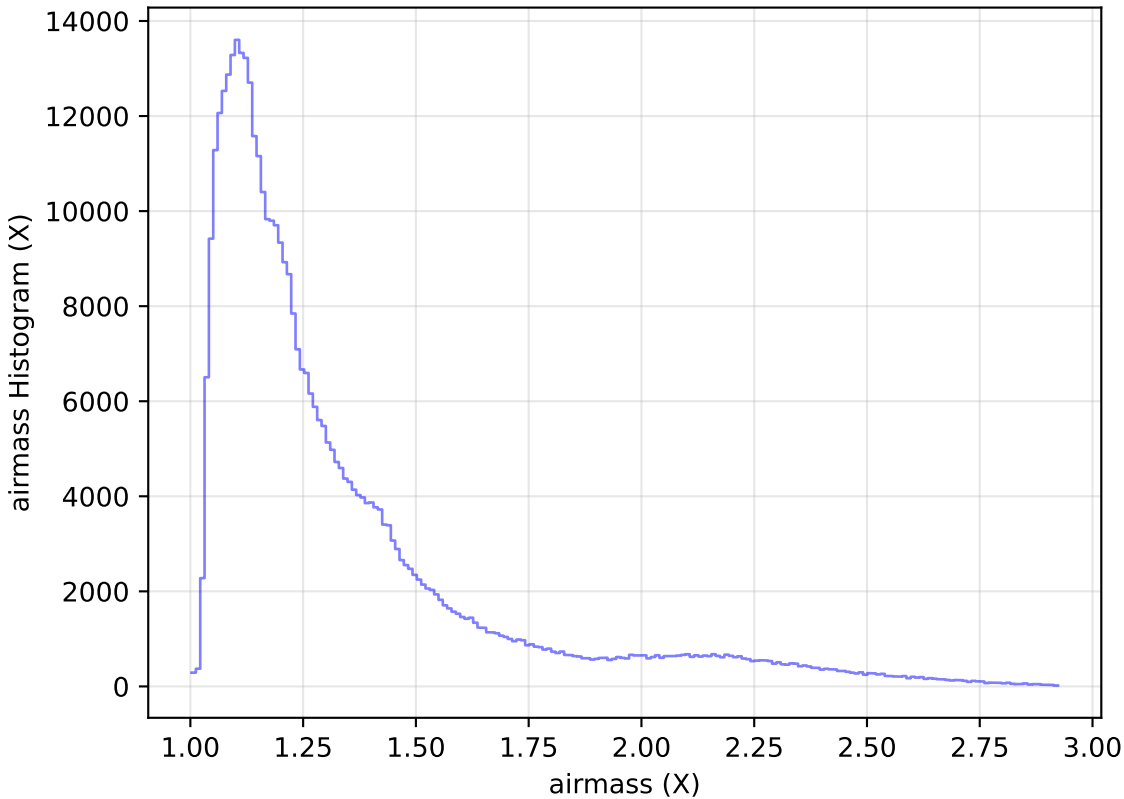
too_elab_heavy_r64_d2_ugrizy_v3.4_10yrs WFD z band: airmass Histogram
